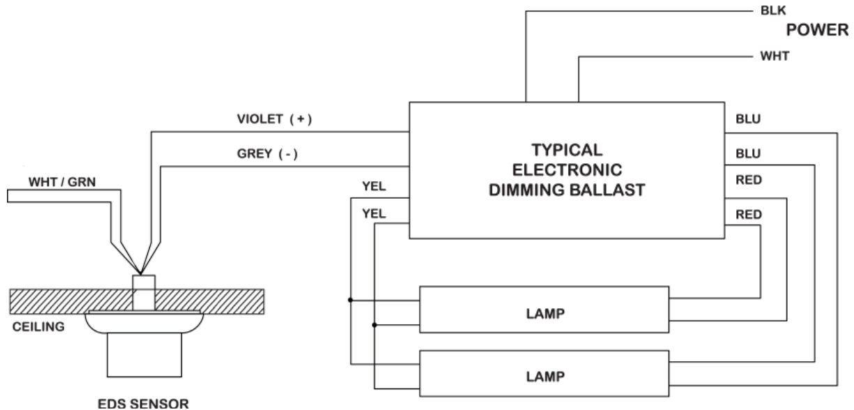
FIGURE 1: CONNECTION DIAGRAM
