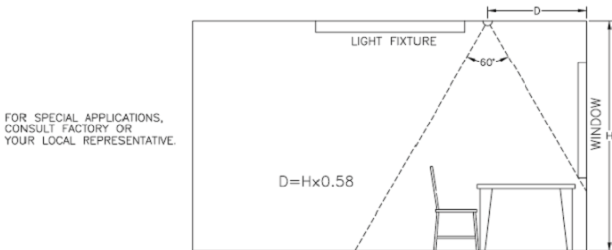
FIGURE 2: SENSOR MOUNTING LOCATION
